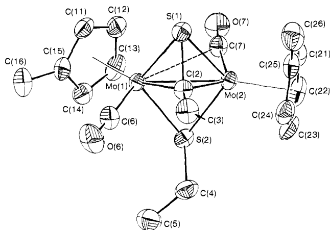
Figure 1. ORTEP diagram of [(\text{CH}_3\text{C}_2\text{H}_4)_2\text{Mo}_2(\text{CO})_2(\text{SCCH}_3)(\text{SC}_2\text{H}_5)] ( 5 ) showing the atom-labeling scheme. Thermal ellipsoids show 50% probability levels and hydrogen atoms have been deleted, here and in Figure 3.
