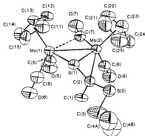
Figure 3. ORTEP diagram of [\text{Cp}_2\text{Mo}_2(\text{CO})_4(\text{CH}_3\text{C}(\text{S})\text{SC}_2\text{H}_5)] ( 6 ) showing the atom-labeling scheme.
