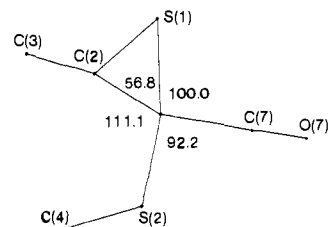
Figure 2. View down the Mo(1)–Mo(2) vector showing dihedral angles (deg) between planes of the type Mo(1), Mo(2), X (esd's < 0.1°).
